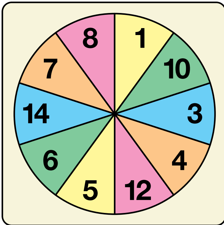
Bits (ones)
