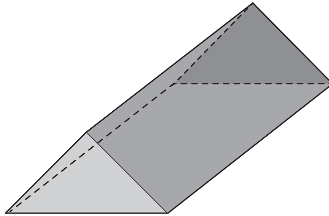
triangular prism
